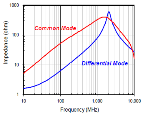
CMX05GYT900F Impedance vs. Frequency
