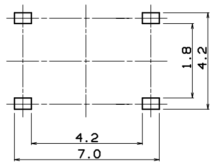
PCB DIMENSION
