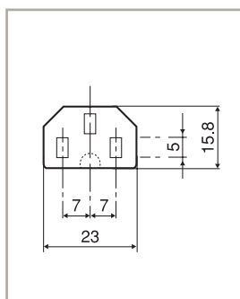
7 - L0 IEC320-C13/C15
