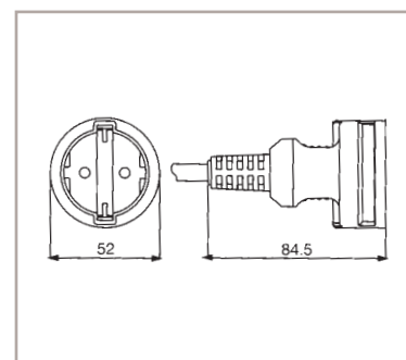
PK95 IEC 60884
