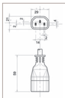
SK 87 EN60320 -1
