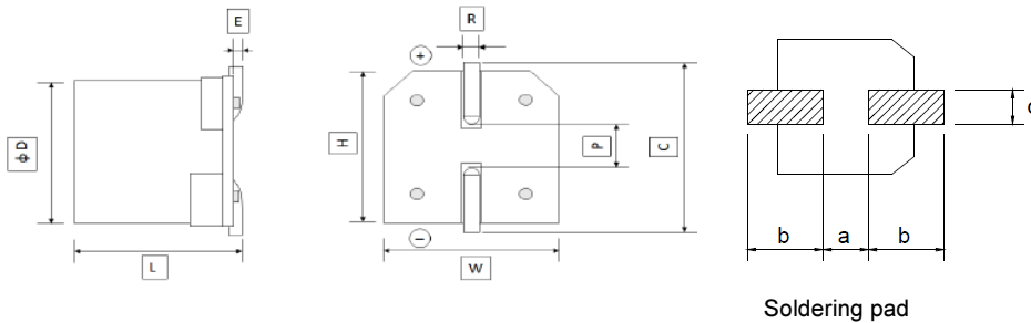
Soldering pad
