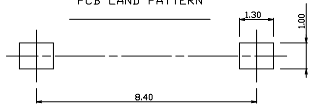
PCB LAND PATTERN
