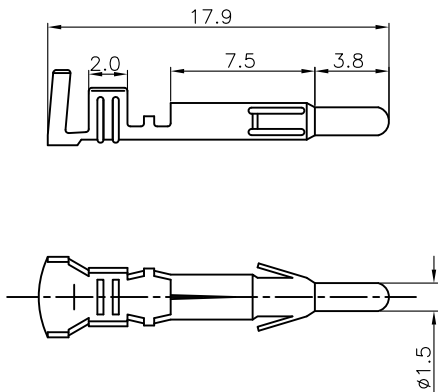
Male TERMINAL
