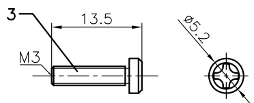
SCREW
