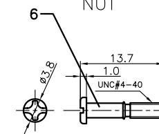
Short BOLT
