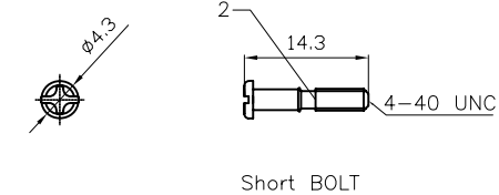
Short BOLT
