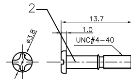
Short BOLT
