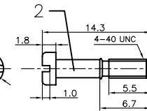
Short BOLT
