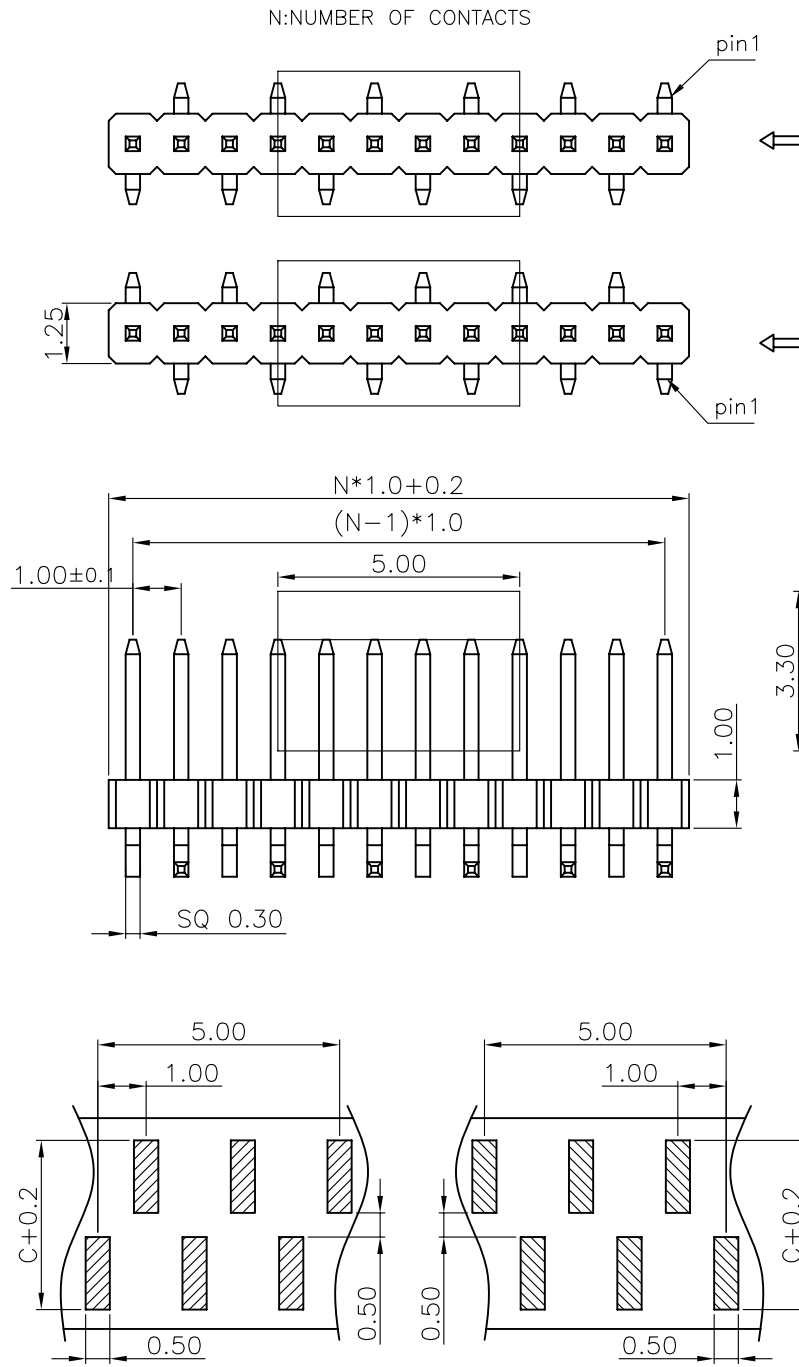
RECOMMEND PCB LAYOUT(R2 TYPE) (TOLERANCE=±0.05) RECOMMEND PCB LAYOUT(R1 TYPE) (TOLERANCE=±0.05)
